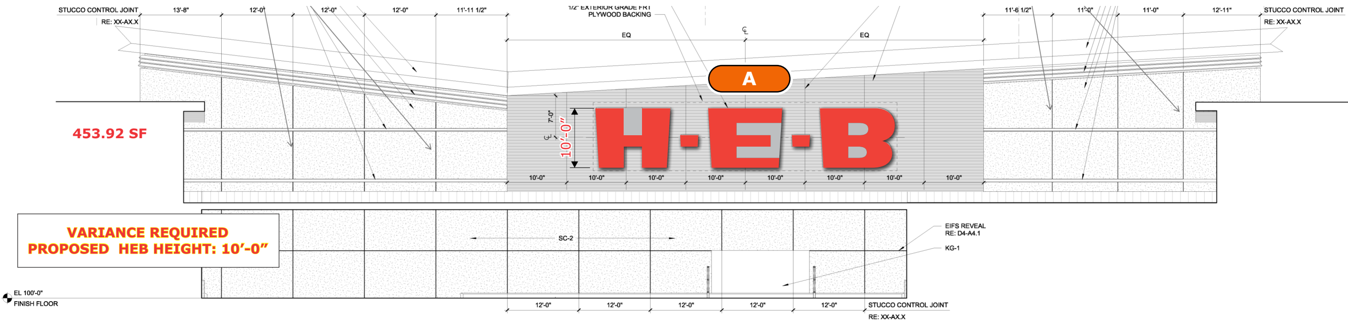
A 10'-0" HEIGHT - FRONT ELEVATION (SOUTH) - ENLARGED AREA Scale: 1/16" = 1'-0"
