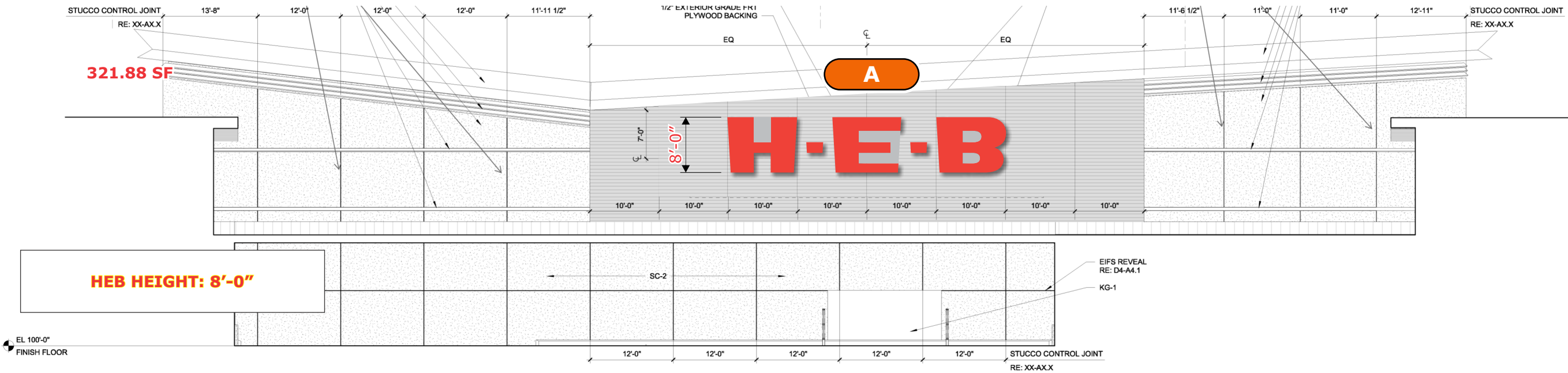
A 8'-0" HEIGHT - FRONT ELEVATION (SOUTH) - ENLARGED AREA Scale: 1/16" = 1'-0"
