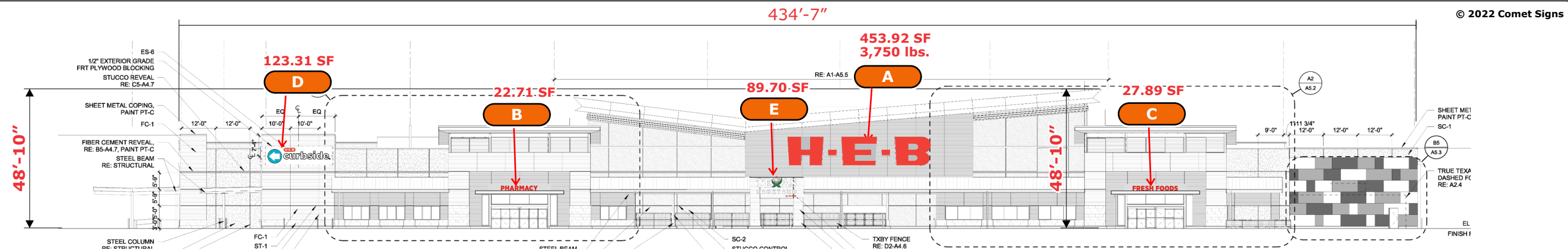
FRONT ELEVATION (SOUTH)
